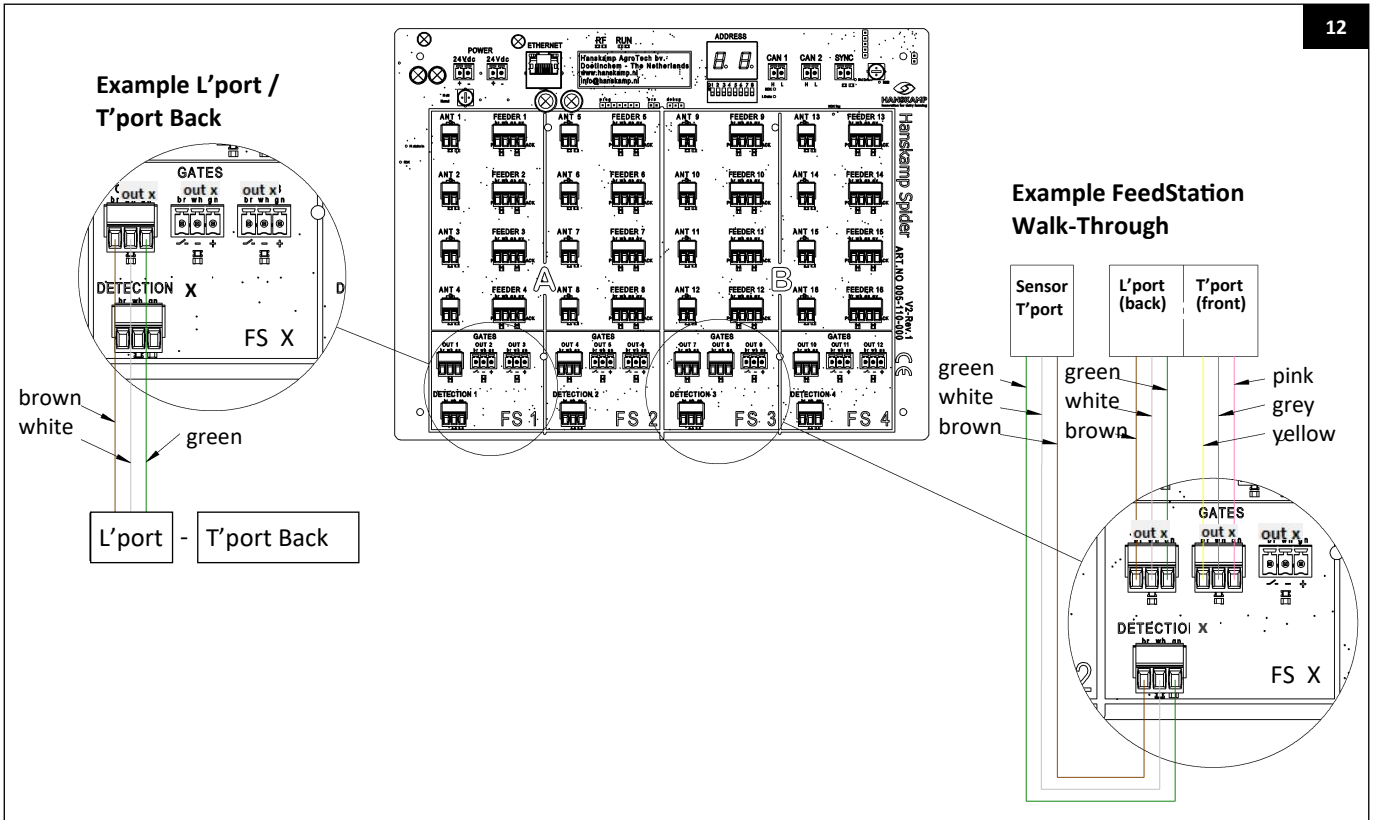
L'port connection diagram (control unit art. no. 002-480-001). If the switch works the other way around, rotate it by 180 degrees.
