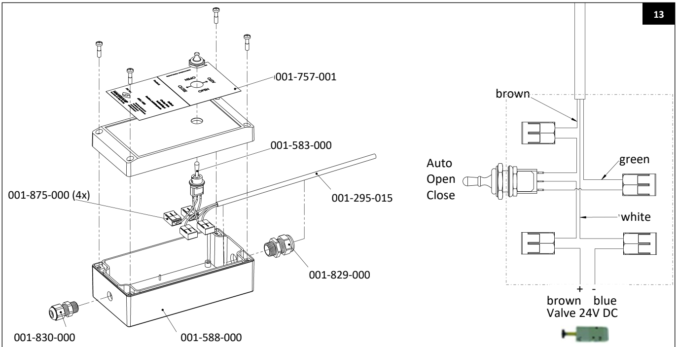
L'port connection diagram (control unit art. no. 002-480-001). If the switch works the other way around, rotate it by 180 degrees.
